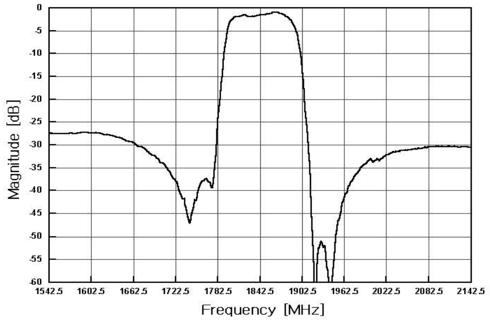
Frequency Response
